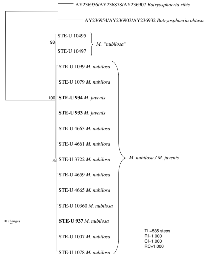
Fig. 2. Single most parsimonious tree obtained from a heuristic search with 100 random taxon additions of a combined ITS, elongation factor 1-alpha and \beta -tubulin sequence alignment. The scale bar shows 10 changes and bootstrap replicate values from 1000 replicates are shown at the nodes. The tree was rooted to two Botryosphaeria species.
