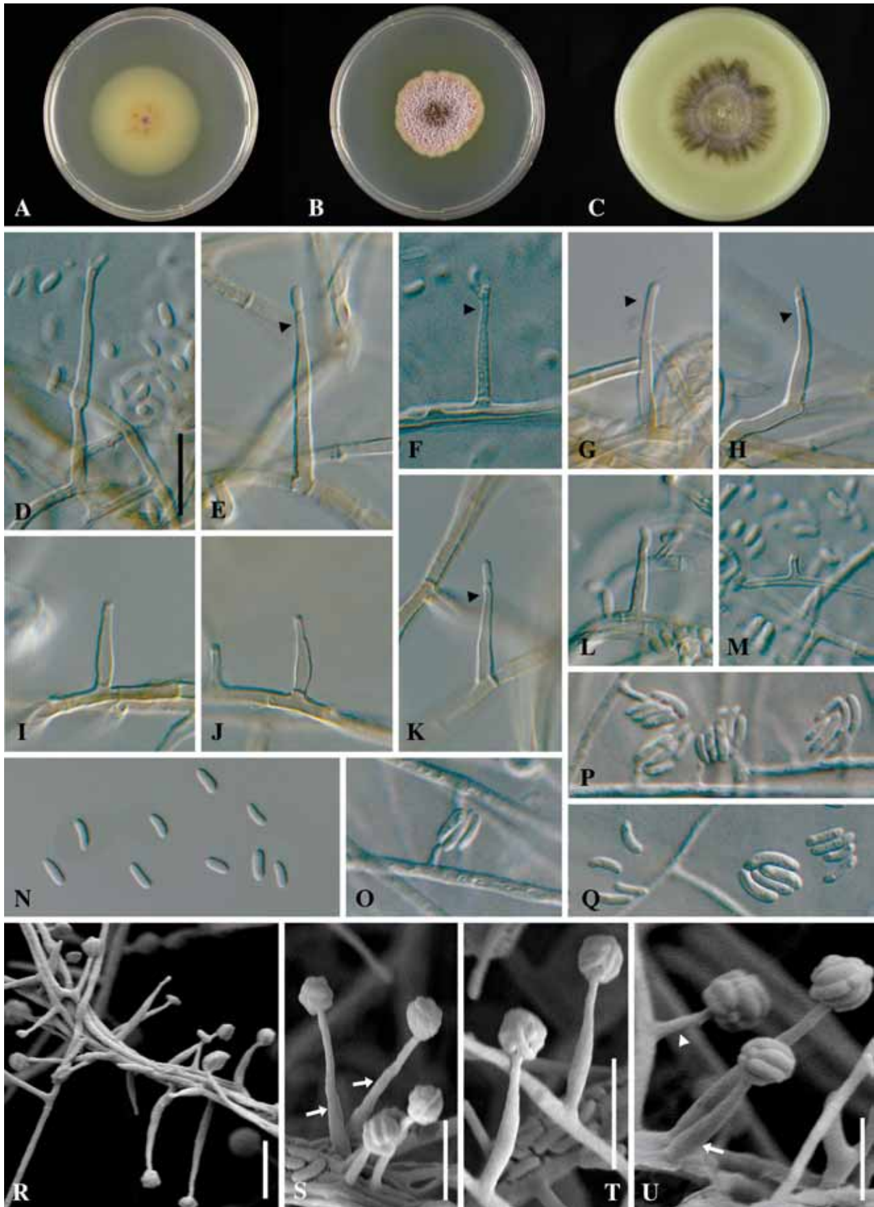
Fig. 41. Phaeocremonium subulatum . A–C. Sixteen-day-old colonies on MEA (A), PDA (B) and OA (C). D–N, R–U. Aerial structures on MEA. D–E. Conidiophores. F–H. Type III phialides. I–L. Type II phialides. Arrow heads indicate subulate apex of phialides (E–H, K). M. Type I phialide. N. Conidia. O–Q. Structures on the surface of and in MEA. O–P. Adelophialides with conidia. Q. Conidia. R. Mycelium with conidiophores and phialides. S. Type III phialides (arrows). T. Type II phialides. U. Type II (arrow) and type I (arrow head) phialides. A–U from CBS 113584. D–Q: DIC; R–U: SEM. Scale bars: D–U = 10 \mu m. Scale bar for D applies to E–Q.
