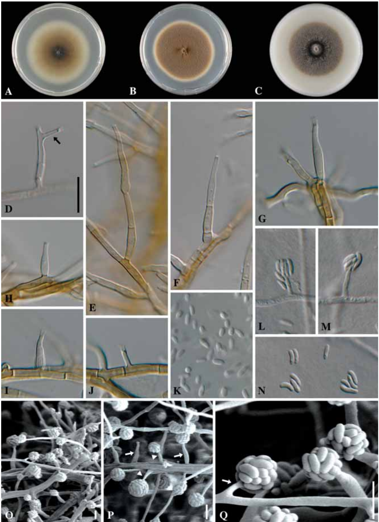
Fig. 21. Phaeoacremonium krajdienii . A–C. Sixteen-day-old colonies on MEA (A), PDA (B) and OA (C). D–K, O–Q. Aerial structures on MEA. D. Conidiophore with polyphialide (indicated by arrow). E–F. Conidiophores. G. Type III phialide. H–I. Type II phialides. J. Type I phialides. K. Conidia. L–N. Structures on the surface of and in MEA. L–M. Adelophialides with conidia. N. Conidia. O. Mycelium and phialides. P. Type II (indicated with arrows) and type I (indicated with arrow heads). Q. Type I phialide (indicated with arrow). A–Q from CBS 109479. D–N: DIC; O–Q: SEM. Scale bars: D–Q = 10 \mu m. Scale bar for D applies to E–N.
