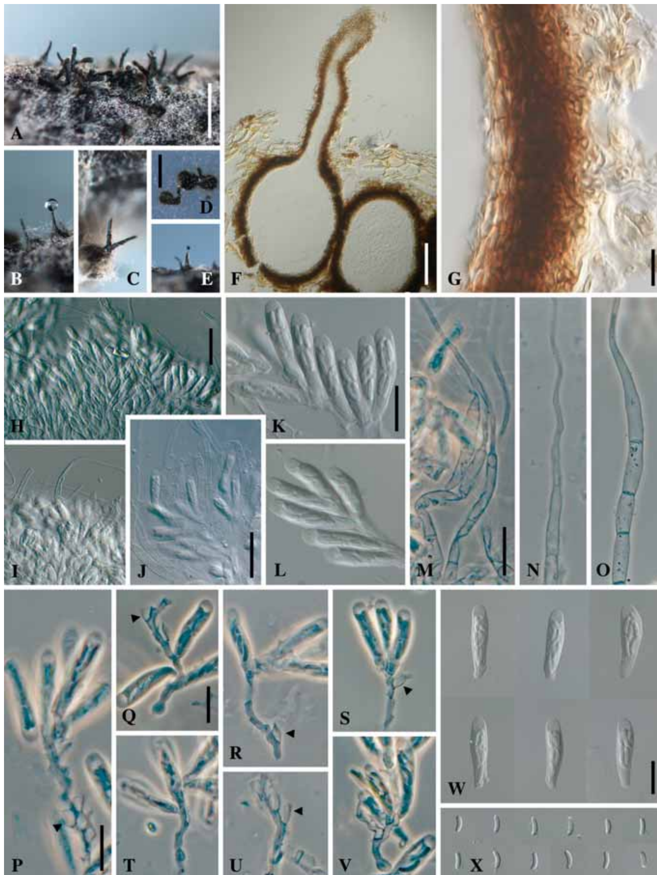
Fig. 20. Togninia krajdenii . A–C, E. Perithecia on canes of Vitis vinifera . D. Perithecia on adjacent water agar. F–G. Longitudinal sections through perithecia; peridium (G). H–J. Asci intermingled with paraphyses. K–L. Asci on ascogenous hyphae. M–O. Paraphyses becoming thread-like towards the tips. P–T, V. Ascogenous hyphae with asci attached; remnant bases indicated by arrow heads (P, Q, R, U, S). U. Ascogenous hypha with remnant bases showing positions where asci were attached. W. Asci. X. Ascospores. A–X from CBS 17460 (holotype). A–E: DM; F–L, W–X: DIC; M–V: PC. Scale bars: A–E = 500 µm; F = 100 µm; H–J = 20 µm; G, K–X = 10 µm. Scale bar for A applies to B–C; bar for H applies to I; bar for K applies to L; bar for M applies to N–O; bar for Q applies to R–V; bar for W applies to X.
