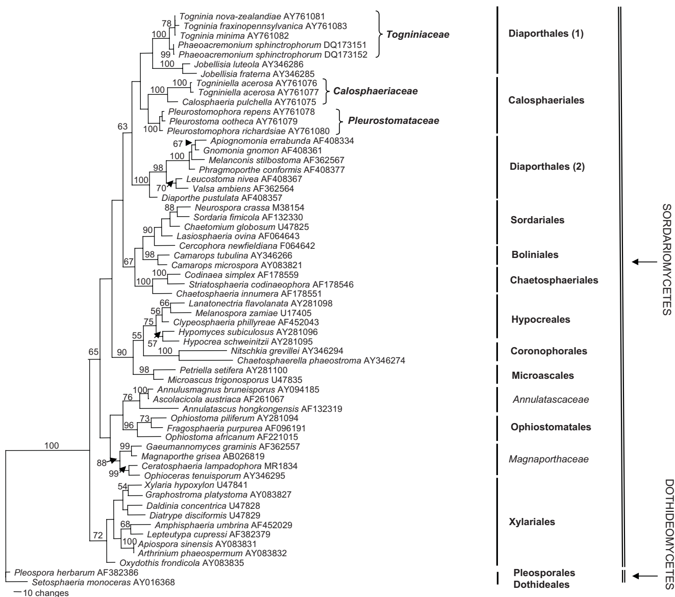
Fig. 9. One of 12 most parsimonious trees obtained from heuristic searches of an alignment of the LSU rRNA gene sequences (TL = 2121 steps, CI = 0.373, RI = 0.643 and RC = 0.240). Bootstrap support values (1000 replicates) above 50 % are shown at the nodes. Pleospora herbarum and Setosphaeria monoceras were used as outgroups. GenBank numbers starting with DQ were newly generated.
