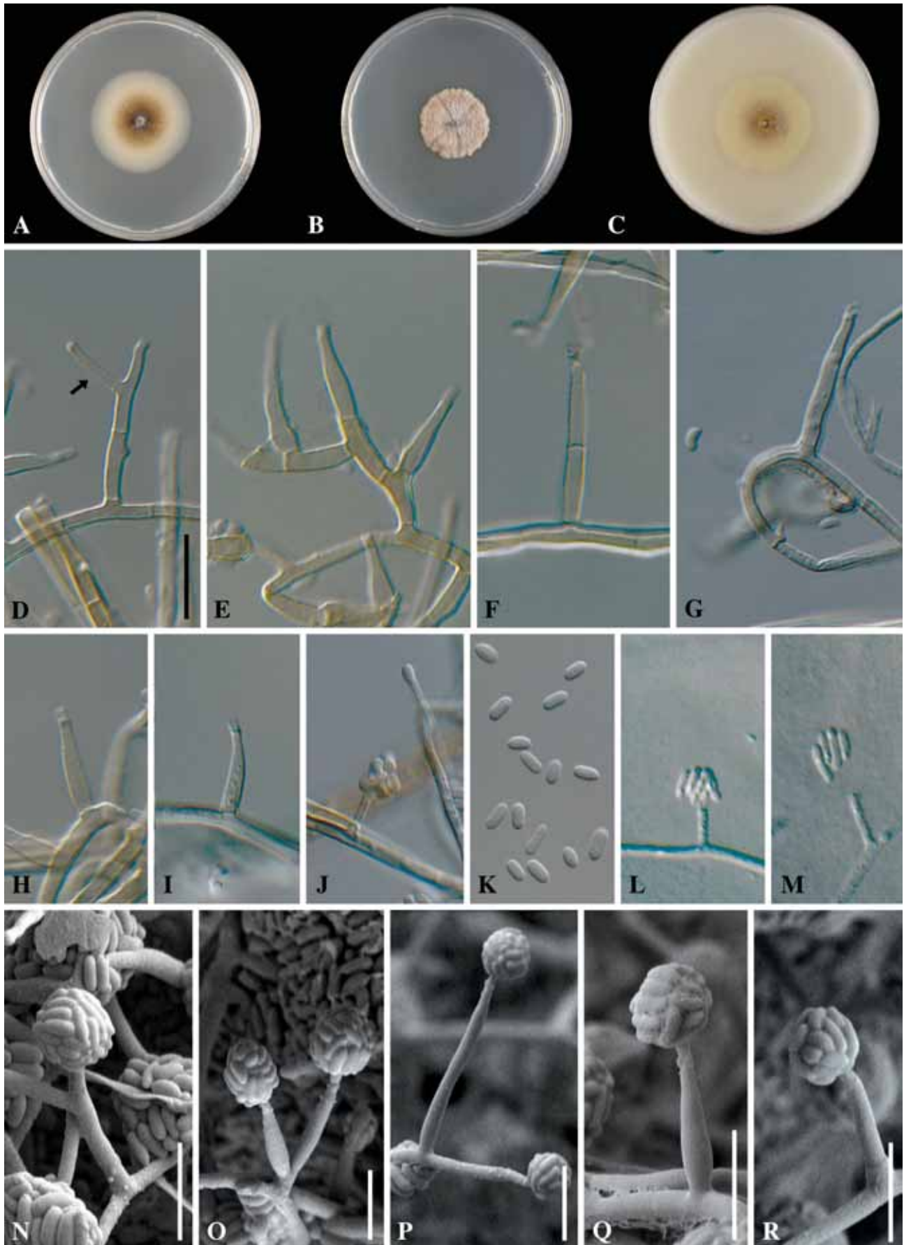
Fig. 35. Phaeoacremonium australiense . A–C. Sixteen-day-old colonies on MEA (A), PDA (B) and OA (C). D–K, N–R. Aerial structures on MEA. D–F. Conidiophores; arrow indicating polyphialide (D). G. Type III phialide. H–I. Type II phialides. J. Type I phialide. K. Conidia. L–M. Structures on the surface of and in MEA. L. Adelophialides with conidia. N–P. Conidiophores. Q. Type II phialide. R. Type I phialide. A–R from CBS 113589. D–M: DIC; N–R: SEM. Scale bars: D–R = 10 \mu m; R = 5 \mu m. Scale bar for D applies to E–M.
