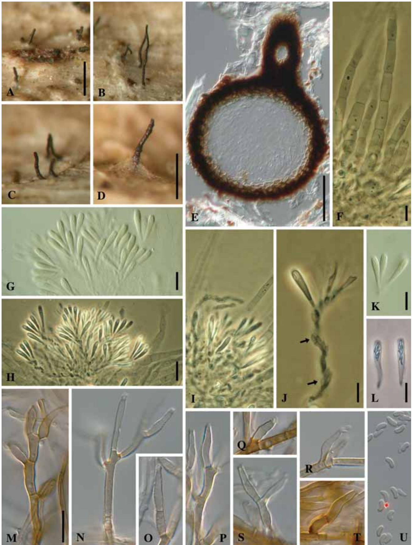
Fig. 51. A–L. Togniniella acerosa , telomorph. A–D. Necks breaking through bark of Nothofagus sp. E. Longitudinal section through perithecium. F. Paraphyses. G–I. Asci attached to ascogenous hyphae intermingled with paraphyses. J. Ascogenous hypha with subtending cells (arrows) from which single asci arise. K–L. Asci. M–U. Phaeocrella acerosa , anamorph. M–P, S–T. Conidiophores. Q–R. Phialides. U. Conidia. A–F, I–L from PDD 81431 (holotype); G, H, PDD 81432 and M–U from ex-type culture CBS 113648 (MEA, 14 d old). A–D: DM, E, G, K, M–U: DIC; F–J, L: PC. Scale bars: A–D = 500 \mu m; E = 100 \mu m; H–I = 20; D, F–G, J–U = 10 \mu m. Scale bar for A applies to B–C; bar for H applies to I; bar for M applies to N–U. Photographs F–L by Réblová.
