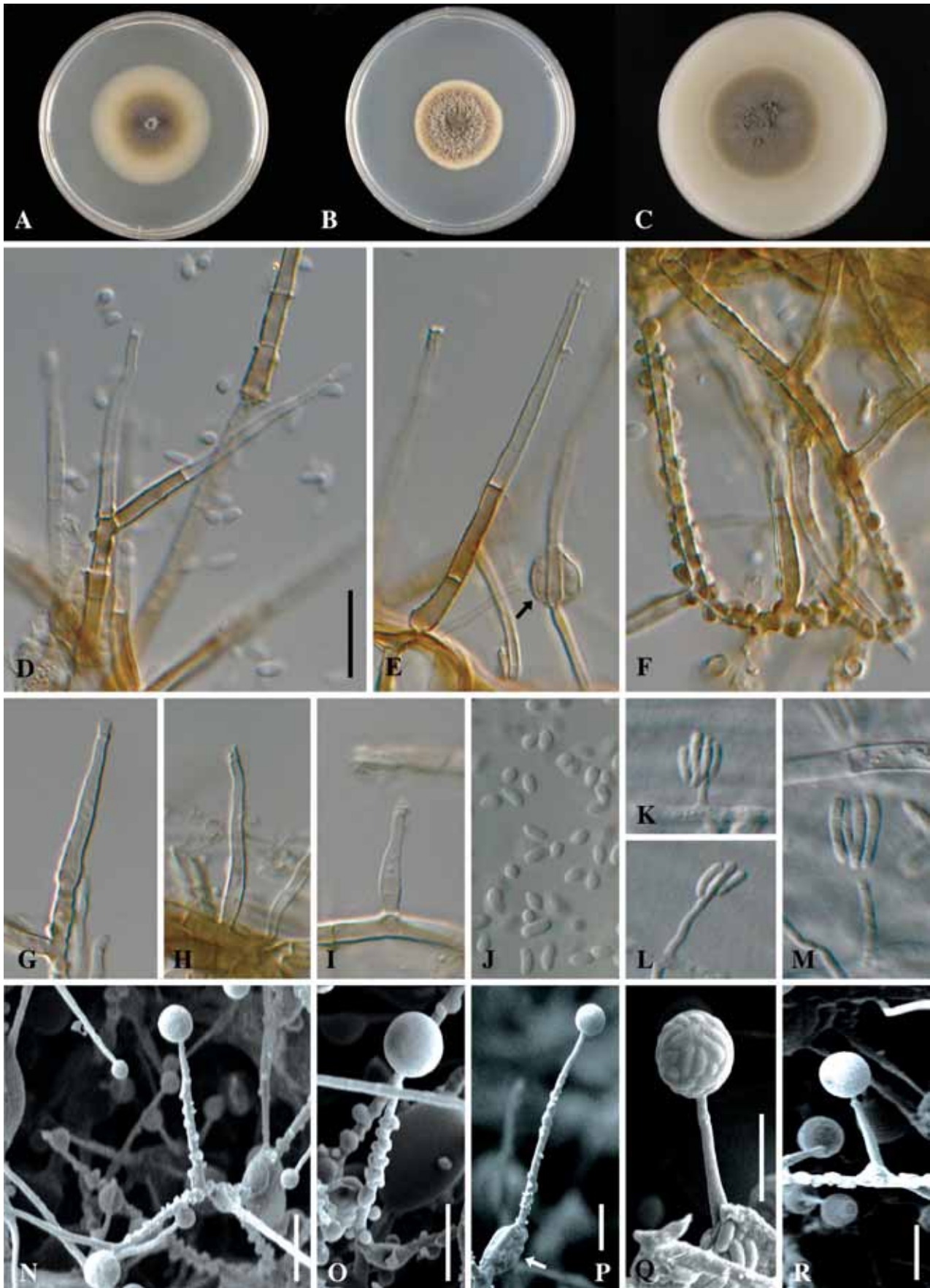
Fig. 27. Phaeoacremonium parasiticum . A–C. Sixteen-day-old colonies on MEA (A), PDA (B) and OA (C). D–J, N–R. Aerial structures on MEA. D–E. Conidiophores; branched conidiophore (D); mucus structures containing conidia commonly found with this species (indicated with arrow; E and P). F. Mycelium showing prominent exudate droplets observed as warts. G–H. Type III phialides. I. Type II phialide. J. Conidia. K–M. Structures on the surface of and in MEA. Adelophialides with conidia. N–O. Type III phialides. P. Conidiophore. Q–R. Type II phialides. A–R from CBS 860.73. D–M: DIC; N–R: SEM. Scale bars: D–R = 10 \mu m. Scale bar for D applies to E–M.
