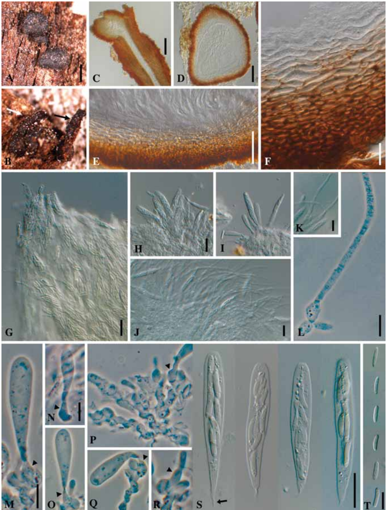
Fig. 48. Calosphaeria vasculosa . A–B. Perithecia underneath the bark of Betula alba ; neck of perithecium indicated by arrow (B). C–F. Longitudinal section through perithecia; apex of a neck (C); asci attached to the inner wall of the peridium (E); peridium (F). G–J. Asci; asci and paraphyses (J). J–L. Paraphyses. M–R. Ascogenous hyphae; immature asci attached to subtending cell on ascogenous hyphae (M–O); subtending cells indicated by arrow heads. S. Asci; short hair-like structure indicated by arrow. T. Ascospores. A–U from holotype PAD, no. 782. A–B: DM; C–K, S, T: DIC; L–R: PC. Scale bars: A–B = 500 \mu m; C–E = 50 \mu m; G–K = 20 \mu m; F, L–T = 10 \mu m. Scale bar for A applies to B; bar for H applies to I; bar for N applies to O–R.
