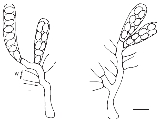
Fig. 3. Ascogenous hyphae of T. viticola with asci and remnant bases still attached [arrows indicate the direction of the length (L) and width (W) measurements as reported in the 'Taxonomy' section]. Scale bar = 10 µm.
