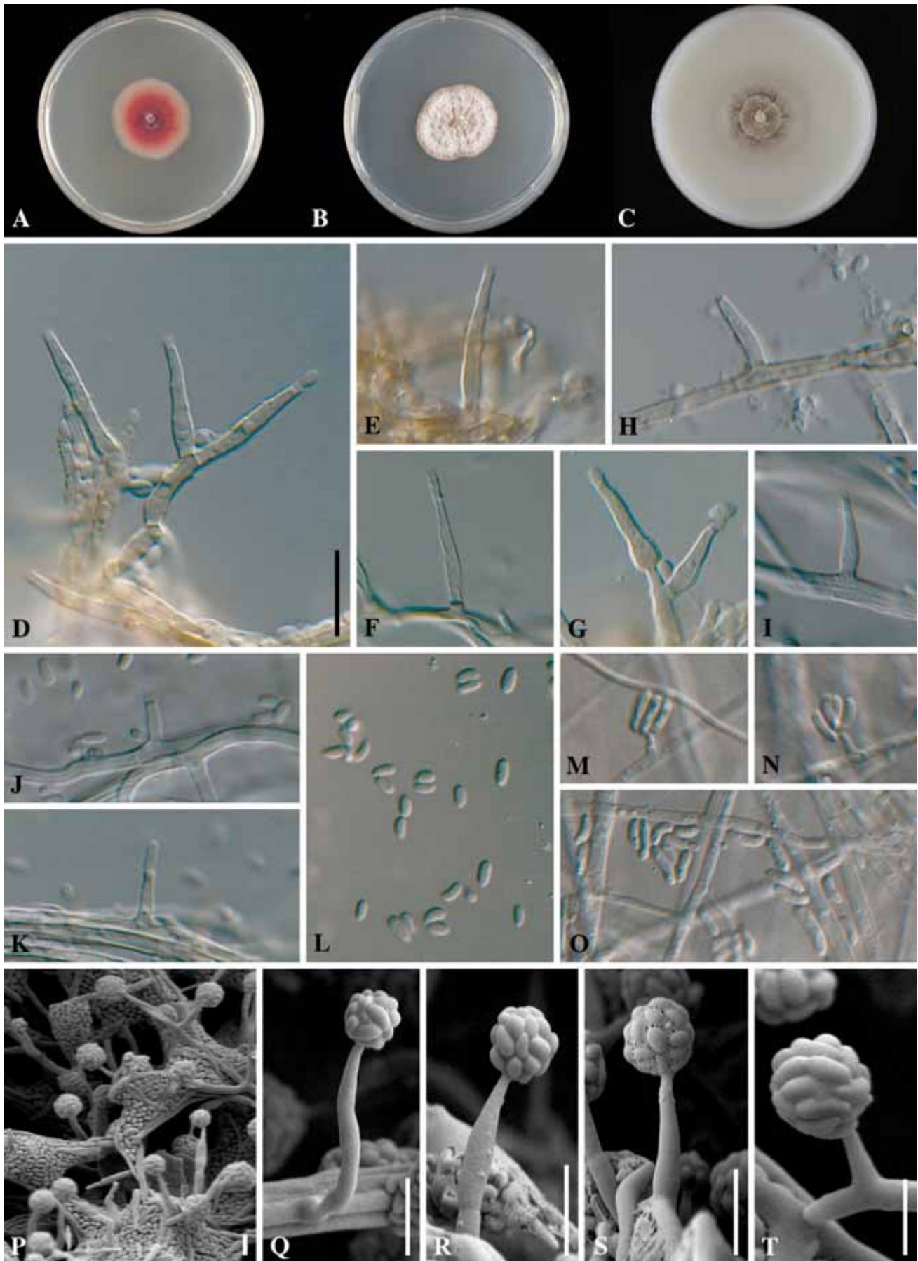
Fig. 36. Phaeocremonium griseorubrum . A–C. Sixteen-day-old colonies on MEA (A), PDA (B) and OA (C). D–L, P–T. Aerial structures on MEA. D. Conidiophore. E–F. Type III phialides. G–I. Type II phialides. J–K. Type I phialides. L. Conidia. M–O. Structures on the surface of and in MEA. M–N. Adelophialides with conidia. O. Conidia. P. Conidiophores and phialides. Q. Type III phialide. R–S. Type II phialides. T. Type I phialide. A–T from CBS 111657. D–O: DIC; P–T: SEM. Scale bars: D–T = 10 \mu m. Scale bar for D applies to E–O.
