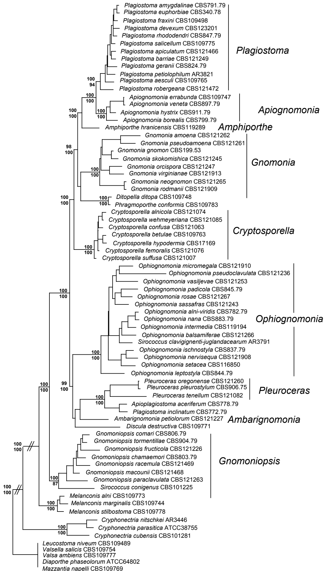
Fig. 1. ML phylogenetic analysis (ML score = -\ln L 26702.18832) of sequences for the tef1 - \alpha , nrlSU and rpb2 multigene analysis of genera in the Gnomoniaceae for 64 gnomoniaceous taxa and 11 outgroup diaporthean taxa. Bayesian posterior probabilities greater than 95 % are shown above each branch. MP bootstrap values greater than 70 % are shown below each branch.
