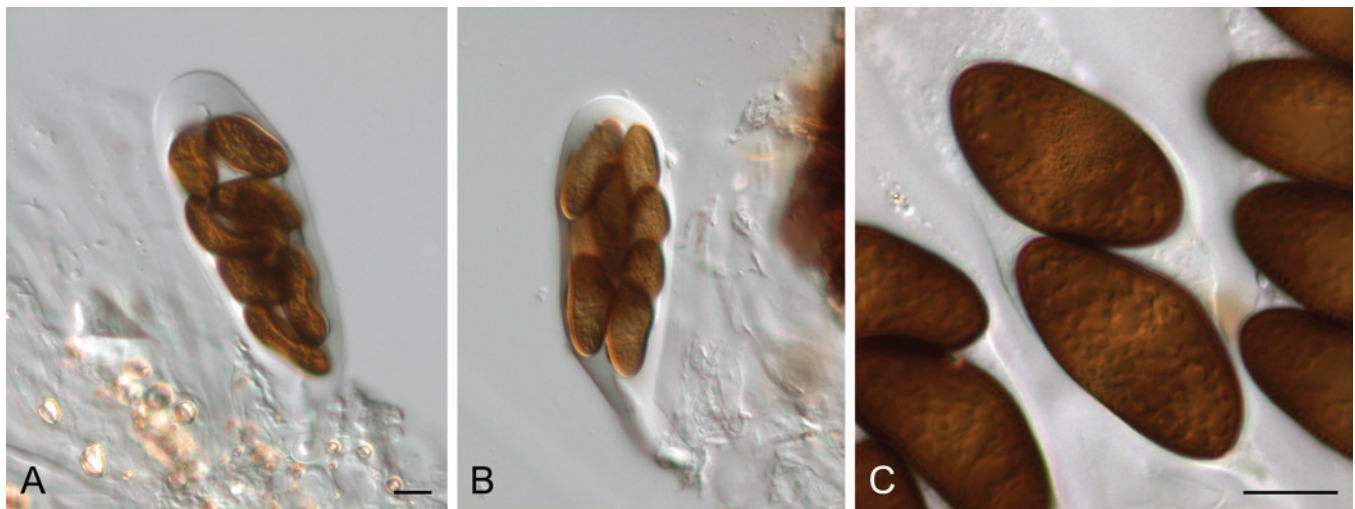
Fig. 65. Sphaeropsis eucalypti . A, B. Asci with ascospores. C. Ascospores. Scale bars = 10 µm. Scale bar in A applies to B.
