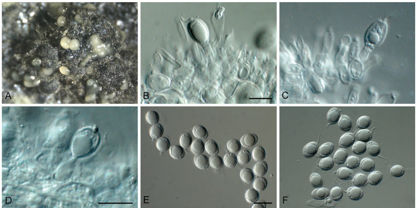
Fig. 6. Phyllosticta concentrica (CBS 937.70). A. Conidiomata sporulating on OA. B–D. Conidiogenous cells giving rise to conidia. E, F. Conidia. Scale bars = 10 \mu m.
