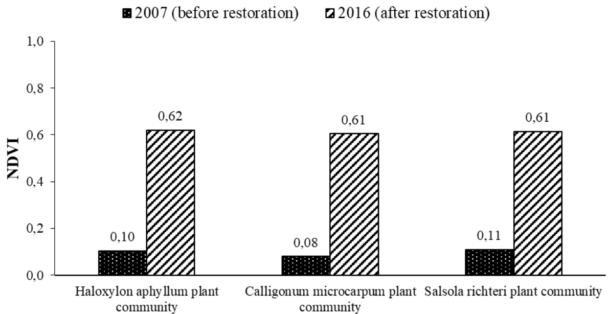
Fig.3.4.1. Dynamics of NDVI values in degraded (2007) and restored (2016) vegetation cover
