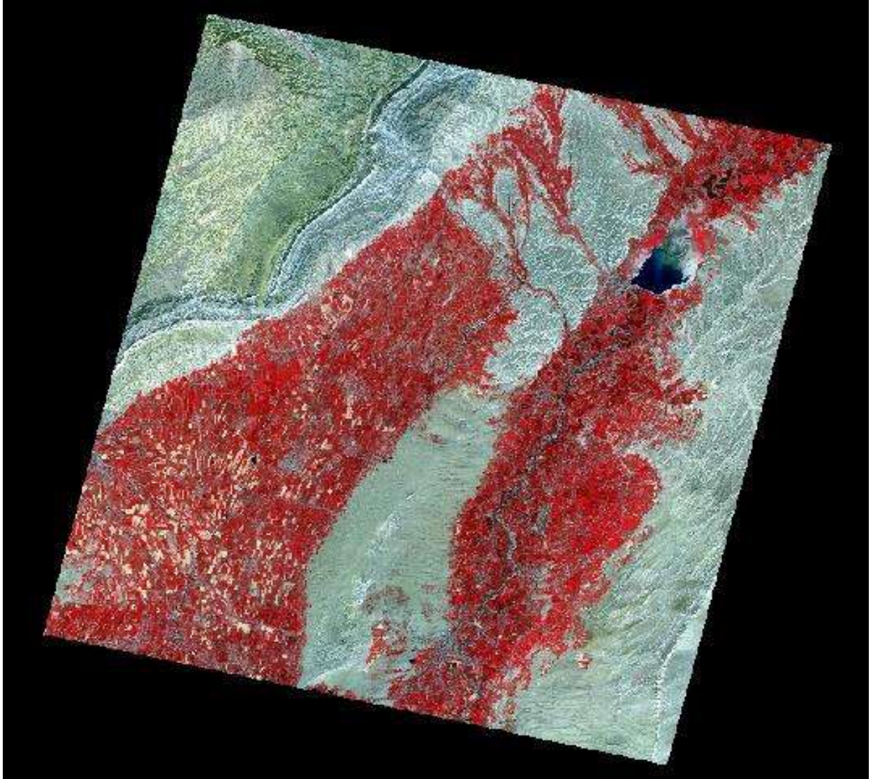
Fig.2.3.3. General view of ASTER image
