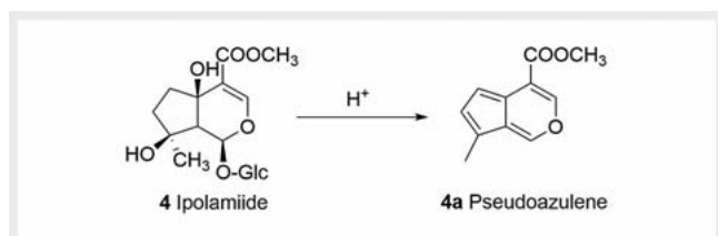
► Fig. 15 Acid-catalyzed degradation of ipolamiide (4) to a fulvouridoid (= pseudoazulene) (4a).
