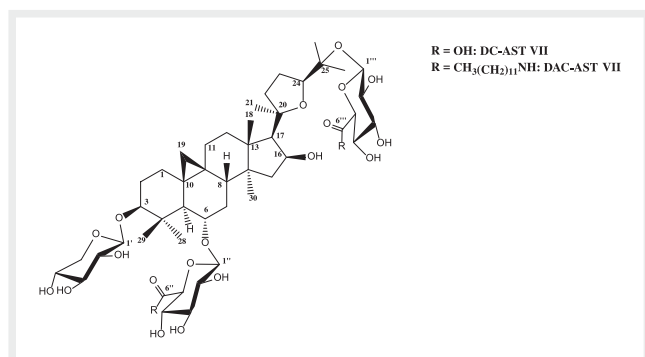
► Fig. 1 Chemical structure of AST VII analogs
