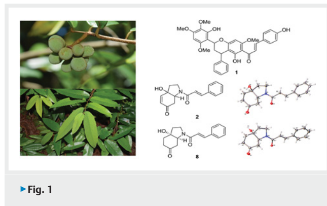
► Fig. 1 Chemical structures of flavonoids 1–23 from the flowers of Coreopsis lanceolata . Glc: O- \beta -D-glucopyranosyl, 6-RG: O- \alpha -L-rhamnopyranosyl-(1 \rightarrow 6)-O- \beta -D-glucopyranosyl.
