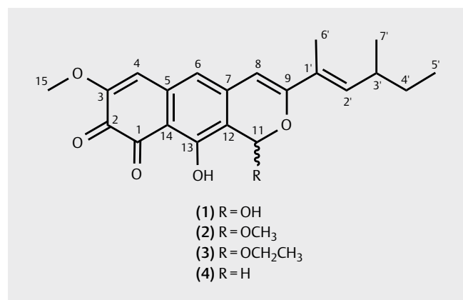
► Fig. 1 Structure of laccaridione C ( 1 ), the related laccaridiones A ( 2 ) and B ( 3 ), and leptosphaerodione ( 4 ).
