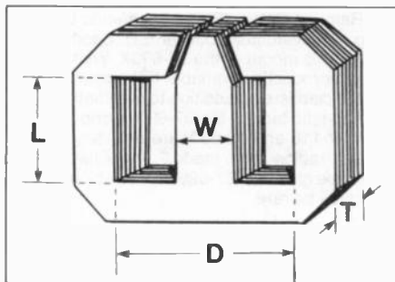
Figure 1. One-piece transformer laminations.
