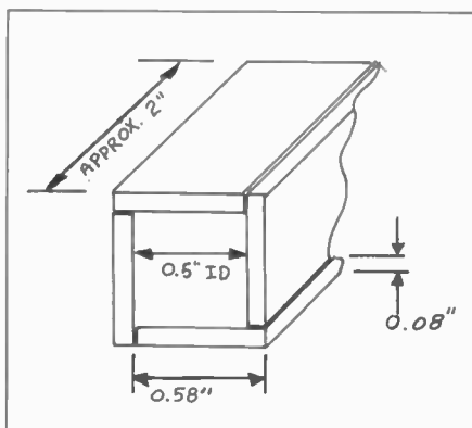
Figure 2. View of the rectangular section of the bobbin.
