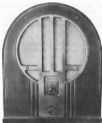
PHILCO MODEL 84B – Philco squeezed quite a good performance from this little 1934 superhet, considering that it uses only 4 tubes, a Type 77 1st detector/oscillator, a Type 77 1F/2nd detector, a Type 42 audio output, and a Type 80 rectifier. The single IF stage uses regeneration to increase sensitivity. (Bill Harris – Roanoke, TX)
