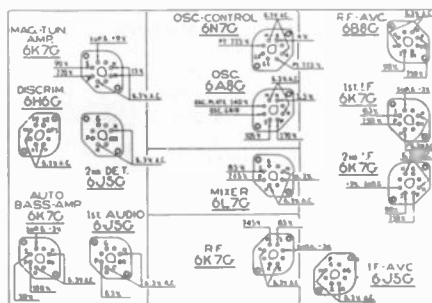
Figure 5. Tube layout for the receiver chassis, mounted on top shelf of cabinet, showing tube layout.
