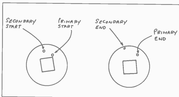
Figure 5. Flanges with typical hole locations.
