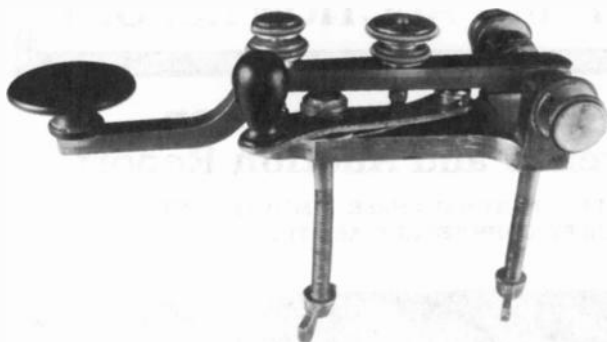
PHILLIPS CURVED LEVER KEY – Patented on May 25, 1880, by Walter P. Phillips, this key features removable iron contacts and an unusual arrangement of the pivot, gap adjustment, contact and spring functions. More details are given in AWA's Old Timer's Bulletin , August 1993, in "Key and Telegraph," edited by Roger Reinke. (John Kelly – Ashton, MD)
