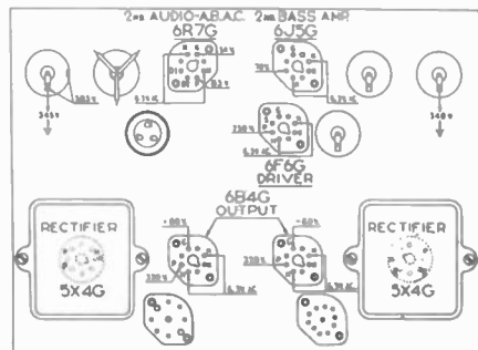
Figure 4. Tube layout for the power unit, containing power supply and audio output. Chassis is located on bottom shelf of cabinet.
