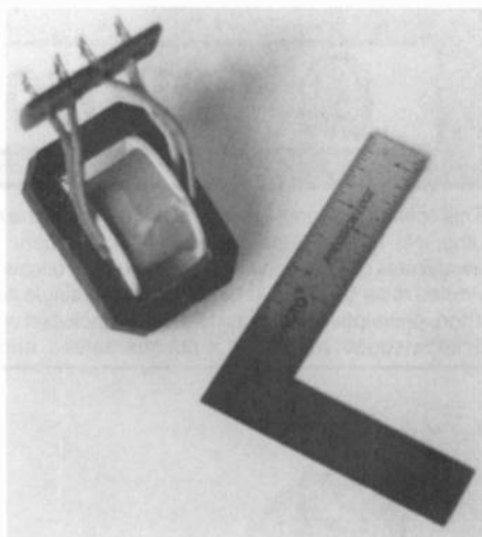
Figure 8. A rewound, rewired transformer ready for installation of the channel frame.
