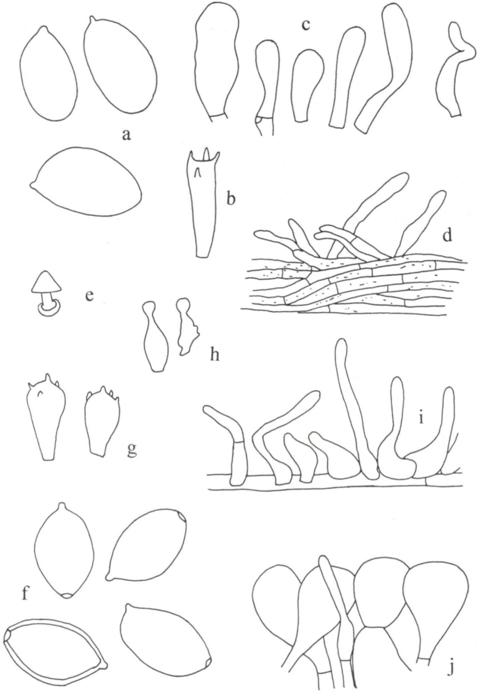
Fig. 13 a-d. Agaricus liratus (type). a Spores, b basidium, c cheilocystidia, d pileipellis. e-j. Galerula locellina (type). e young fruitbody redrawn from a drawing of MURRILL (x 0.8), f spores, g basidia, h cheilocystidia, i stipe covering, j pileipellis.
