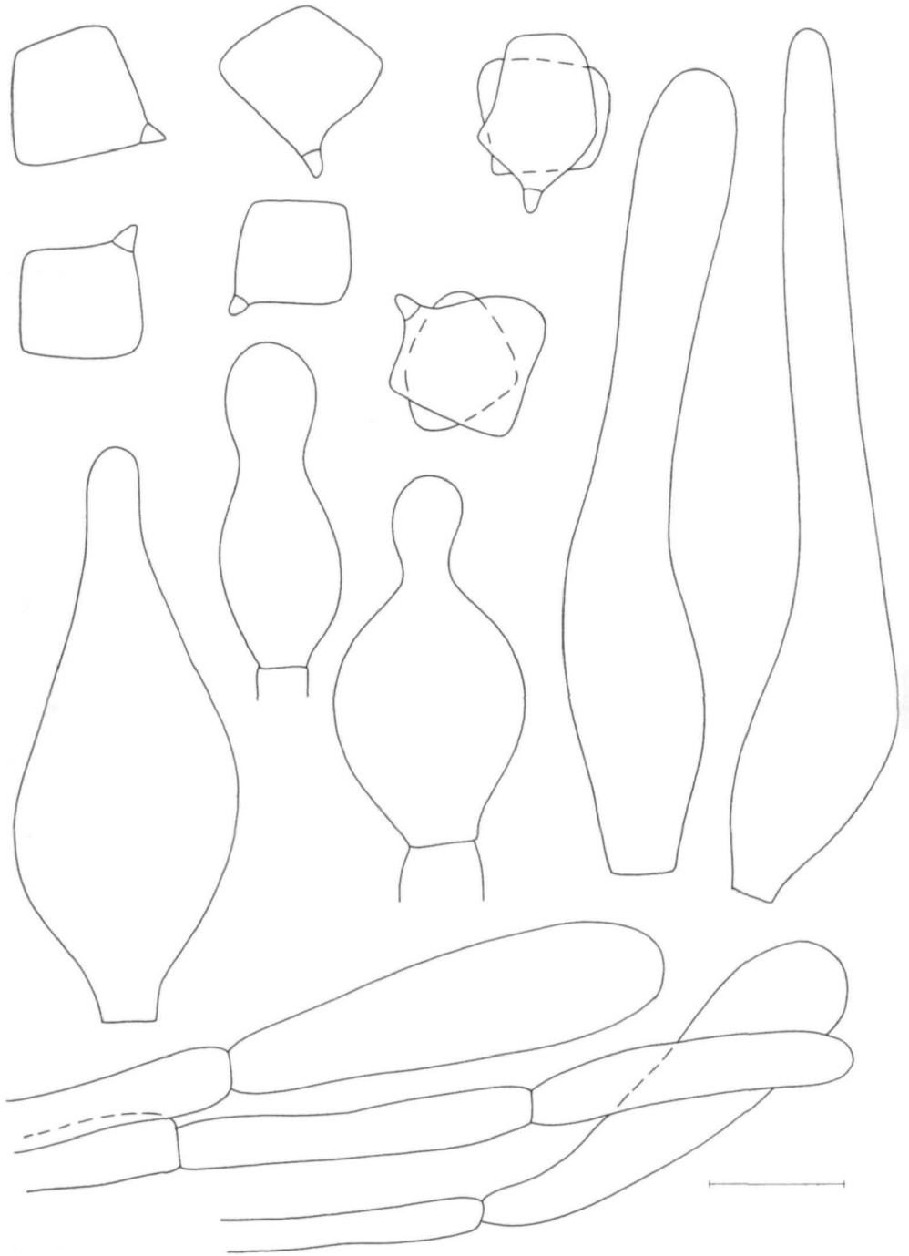
Fig. 44. Agaricus watsonii . Spores, cheilocystidia, pleurocystidia and pileipellis. – Bar: 10 \mu m (spores), 20 \mu m (all other figs.).
