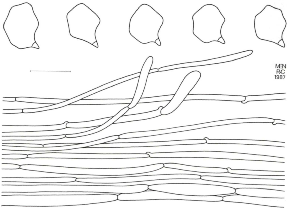
Fig. 18. Entoloma grande . Spores and pileipellis. – Bar: 10 \mu\text{m} (spores), 20 \mu\text{m} (all other figs.).
