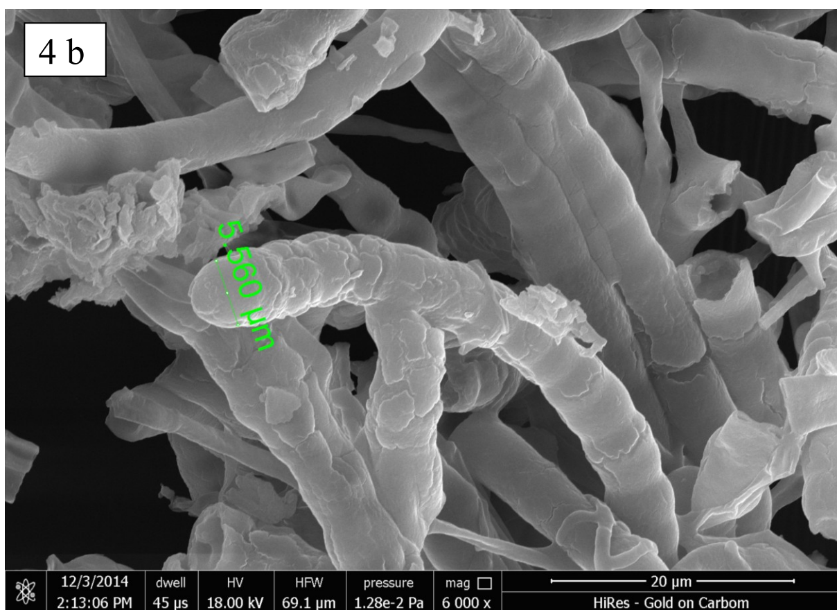
Fig. 4. SEM images of Helicoceras celtidis , a conidia at 3000 \times , b conidia, conidial cell width of 5.5 \mu\text{m} and bursting of conidia, 6000 \times , c mycelium clustering, 3000 \times , d , e attachment to the host at 800 \times and 1600 \times , respectively
