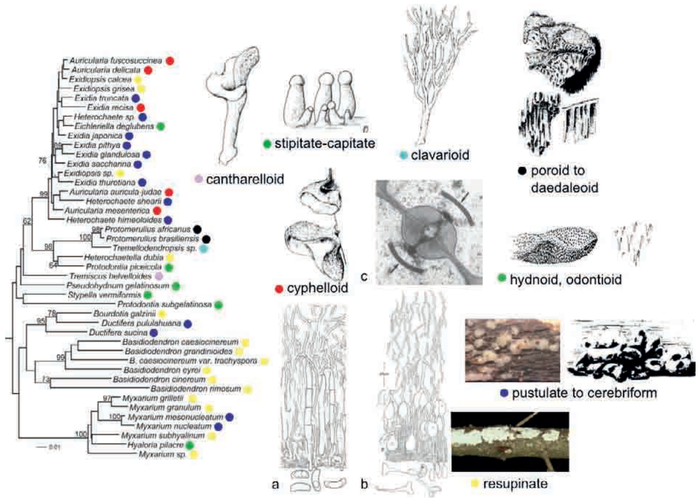
Fig. 41: Macro- and micromorphology of basidiocarps, dolipore with parentheses and phylogenetic hypothesis for representative species and genera of the Auriculariales. a Auricularia auricula-judae , b Exidiopsis effusa , c dolipore with continuous parentheses. The colored dots in the dendrogram refer to positions of species and genera in the phylogenetic tree. Neighbour-joining analysis of an alignment of nuclear DNA coding for the 5 terminal domain of the 28 S ribosomal large subunit. Genetic distances were computed according to the KIMURA two-parameter model. Branch lengths are scaled in terms of expected numbers of nucleotide substitutions per site. Dendrogram from WEISS & OBERWINKLER (2001). Septal pore orig. R. BAUER, illustrations orig. F. OBERWINKLER.
