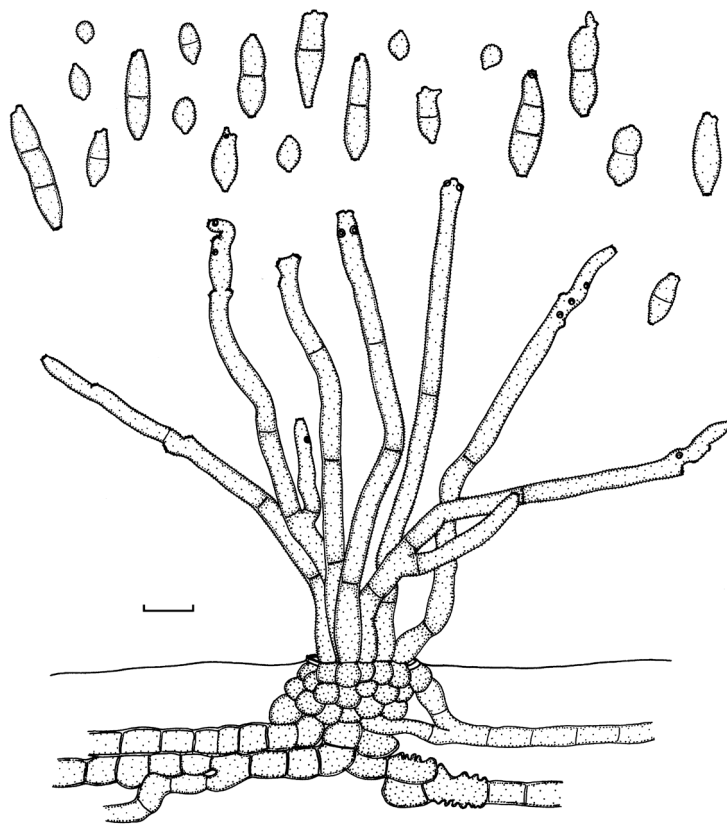
Fig. 4: Cladosporium foliorum (from the holotype). Fascicle of conidiophores and conidia. Bar = 10 \mu\text{m} .
