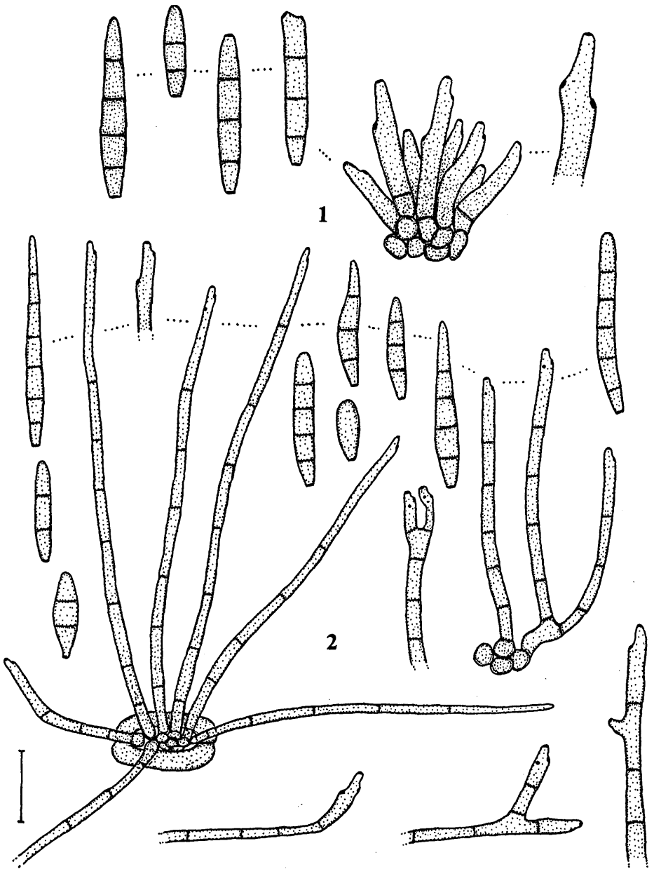
Fig. 1-2: 1 - Phaeoramularia occidentalis (type of Cercospora cassiicola ), fascicle of conidiophores, conidiophore, conidia; 2 - Mycovellopsiella consimilis , fascicles of conidiophores, conidiophores, creeping hyphae, conidia; scale = 20 \mu m; U. Braun del.
