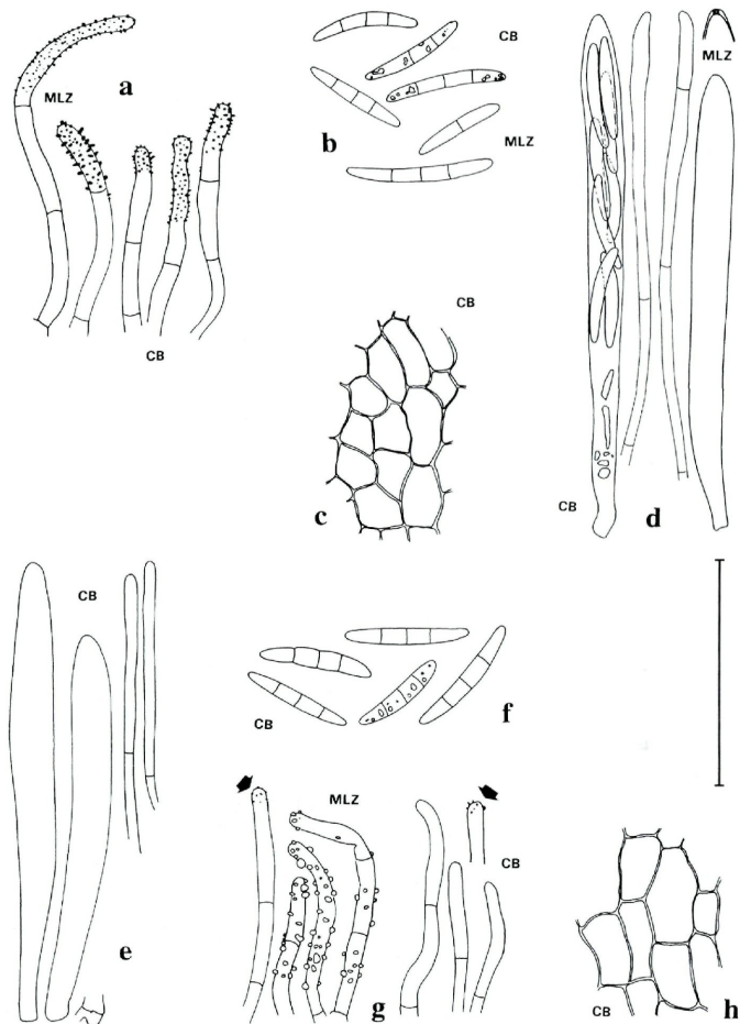
Fig. 2. – Cistella tenuicula , SH 87/147 (a–d) and topotype of Peziza tenuicula (e–h). – a. hairs; b. spores; c. ectal excipulum; d. asci and paraphyses; e. asci and paraphyses; f. spores; g. hairs, showing deforming and stable (arrows) warts; h. ectal excipulum. Scale 50 \mu m.
