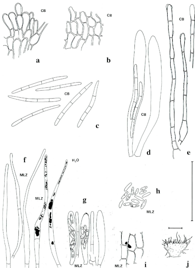
Fig. 1. – a–e: Arachnopeziza delicatula . – a. margin; b. ectal excipulum; c. spores; d. asci; e. hairs. – f–j: A. variopilosa . – f. hairs showing the resinous contents; g. asci and paraphyses; h. spores; i. ectal excipulum showing the amyloid reaction; j. dry apothecium. – Scale 50 \mu\text{m} , for apothecium 100 \mu\text{m} .
