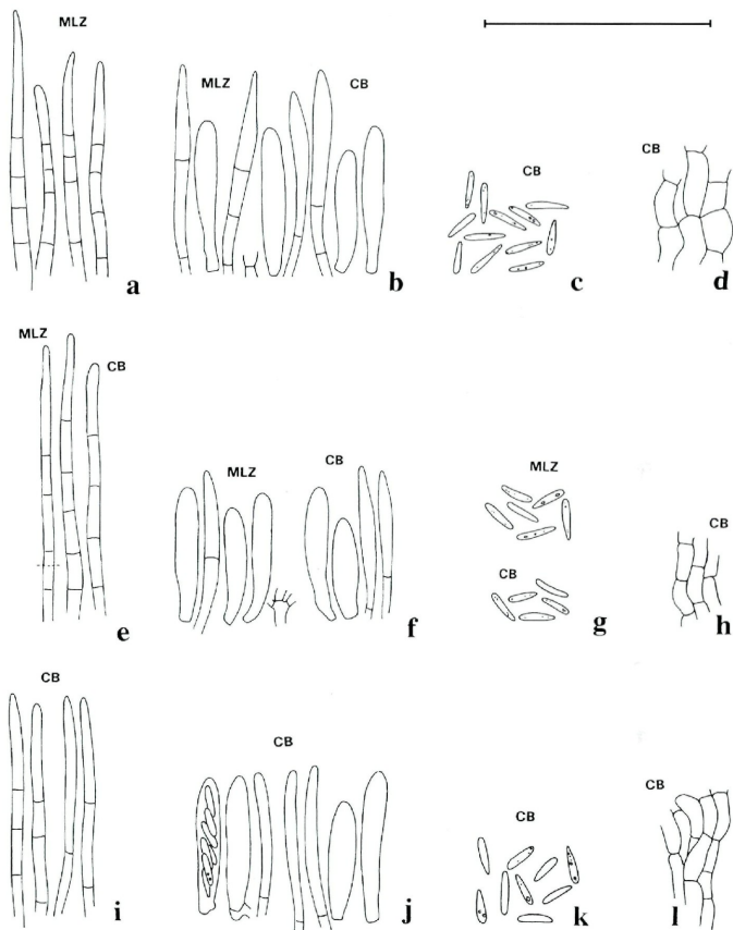
Fig. 4. - Psilachnum acutum , SH 88/125 (a-d), 88/64 (e-h) and 88/23 (i-l). - a, e, i. hairs; b, f, j. asci and paraphyses; c, g, k. spores; d, h, l. ectal excipulum. - Scale 50 \mu m.
