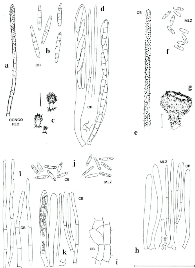
Fig. 3. - a-d. Lasiobelonium belanense . - a. hair; b. spores; c. dry apothecia; d. asci and paraphyses. - e-h. Lachnellula calyciformis . - e. hair; f. spores; g. dry apothecium; h. asci and paraphyses. - i-l. Archnopeziza variepilosa . - i. ectal excipulum; j. spores; k. asci and paraphyses; l. hairs. - Scale 50 µm, for apothecia 100 µm.
