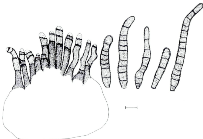
Fig. 11. - Stigmia rhois . Conidia and conidioma with conidiophores and conidiogenous cells showing enteroblastic proliferation (PREM 51132, holotype; bar = 10 \mu\text{m} ).
