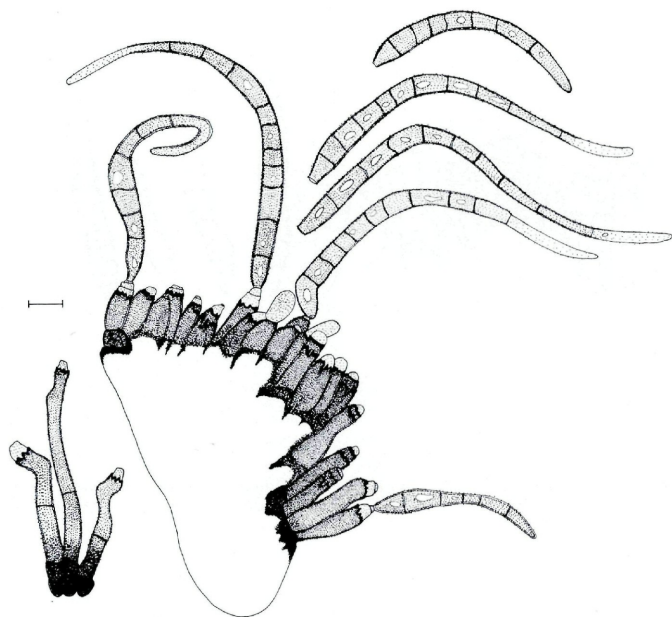
Fig. 10. - Stigmina curvispora . Conidioma with conidiophores and conidiogenous cells showing enteroblastic proliferation, giving rise to curved conidia (PREM 51105, holotype; bar = 10 \mu\text{m} ).
