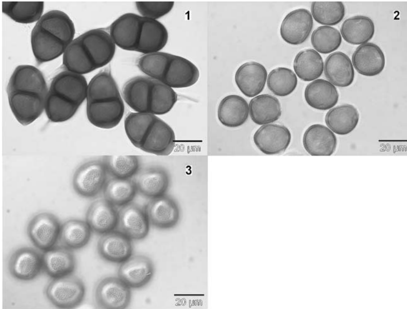
Figs. 1–3. Puccinia ardahanensis : 1. Teliospores. 2. Urediniospores: optical section. 3. Urediniospores: focus on spore surface showing finely and densely verruculose spore wall.
