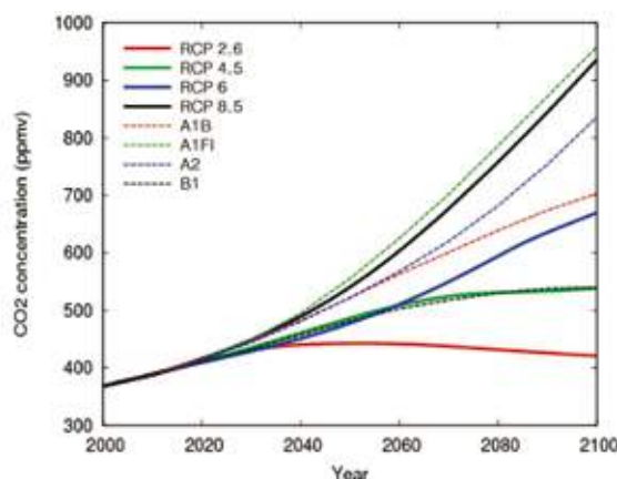
Figure 2.3 Comparison of carbon dioxide ( \text{CO}_2 ) concentrations (ppm), 2000–2100, for the new Representative Concentration Pathways (RCPs), and the previous Special Report on Emissions Scenarios (SRES) scenarios (adapted from Collier et al. 2011).
