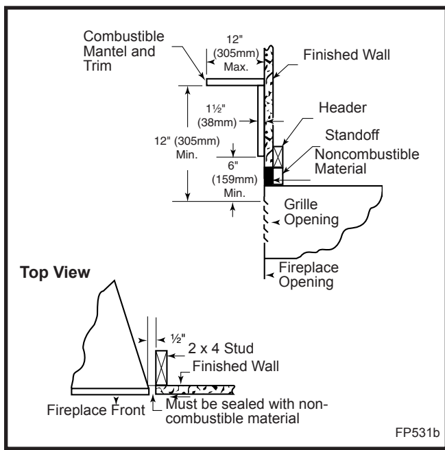
Fig. 22 Mantel clearance.
