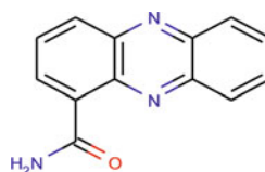
phenazine-1-carboxamide
