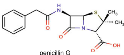
penicillin G
