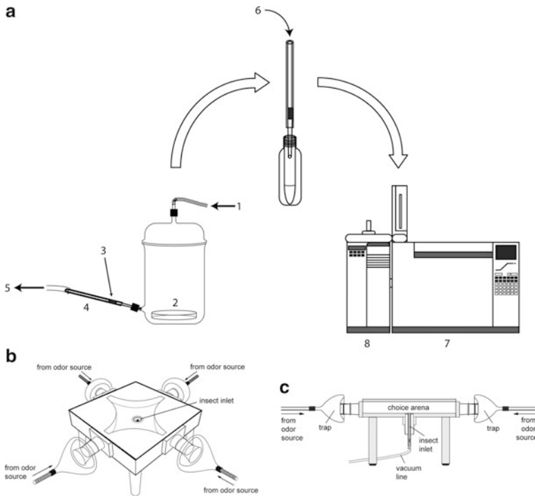
Fig. 1 Apparatus for chemical and biological analysis of volatile organic compounds. (a) Volatile collection system requiring: 1 clean air into the system, 2 test sample, 3 Super-Q packing material to trap volatile chemicals, 4 removable filter containing packing material, 5 vacuum for pulling air through the system, 6 solvent added to filter to remove chemicals from packing material, 7 gas chromatograph where solution with volatile chemicals is injected to separate out the individual chemicals, 8 mass spectrometer and/or FTIR to identify chemicals by characteristic chemical spectra. (b) A four-armed airflow olfactometer that requires a constant stream of purified air guided over each of four odor sources (or blank controls) into a choice arena, into which the test insect is introduced through a central inlet. Orientation and behavior of the insect in the four produced odor fields are recorded for a determined time period and evaluated using Observer XT (Noldus Information Technology) software. (c) Side view of the olfactometer. A central vacuum line directs the airflow and assures the generation of four odor fields in the arena
